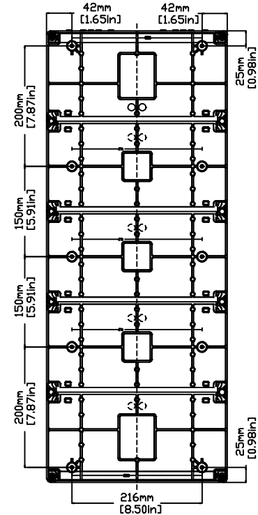
BOTTOM VIEW
